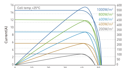
I-V/P-V Curve at different Irradiation (585W)
